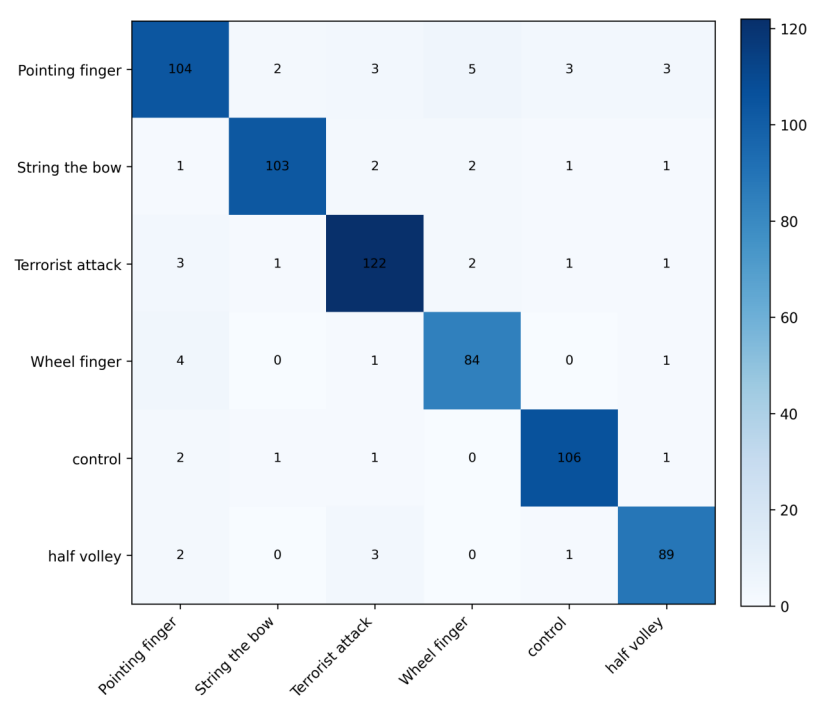
Fig. 5. Posture classification confusion matrix.
