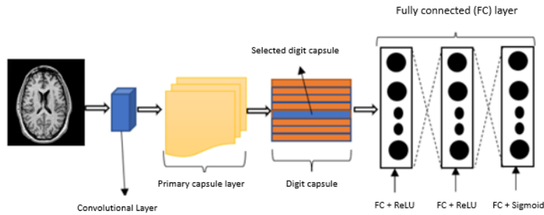
Fig. 7. Illustration of a typical segmentation workflow leveraging Capsule Networks.
