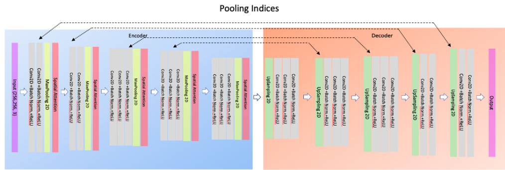
Fig. 2. SEGNET with Spatial Attention Architecture.
